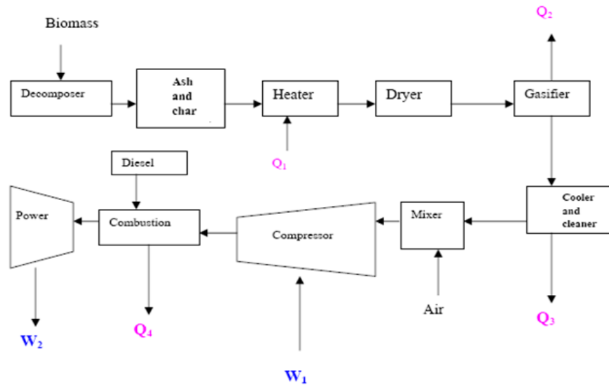
Figure 7. Advanced biomass power with diesel engine (Omer, 2006).
