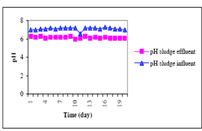
Figure 6. Potential of hydrogen (pH) sludge before and after treatment in the digester (Omer, 2006).
